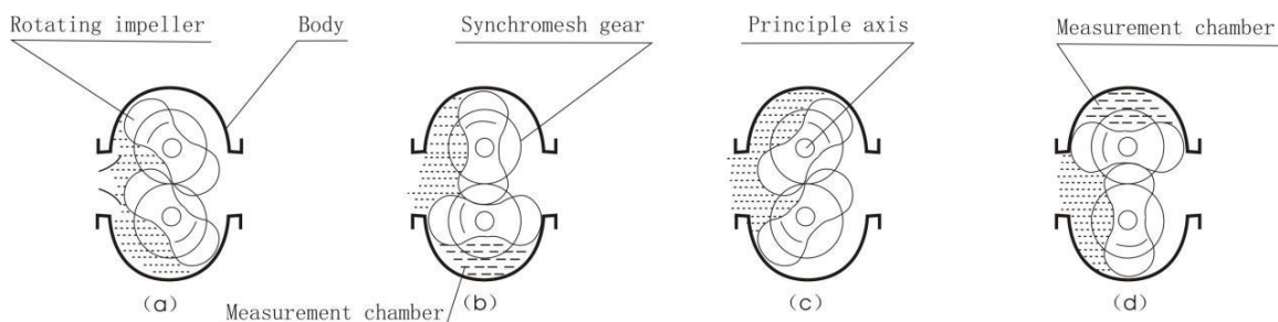
Figure 2 Structure schematic
