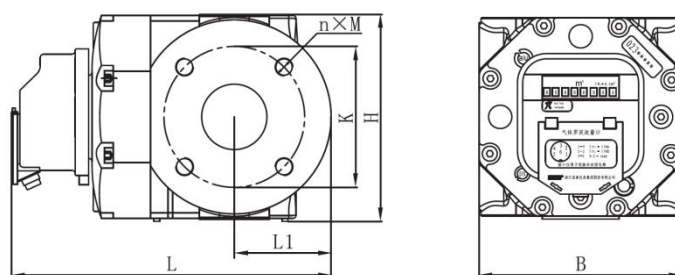
Figure5 Outline structure
