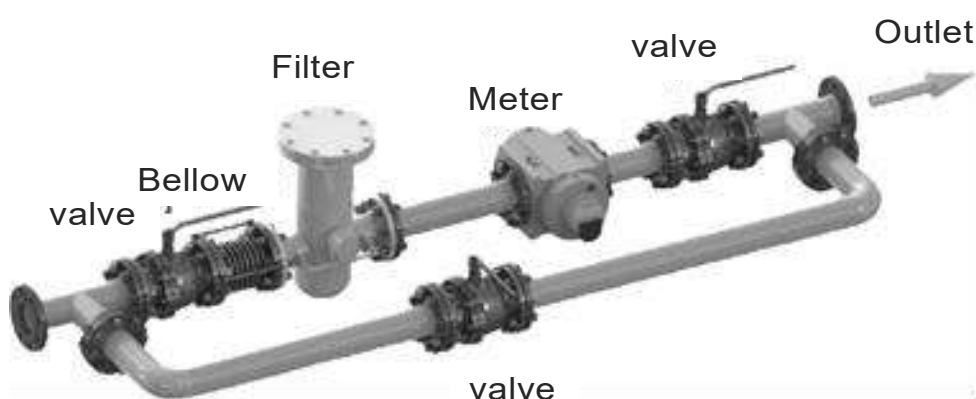
Figure 6 Horizontal installation
