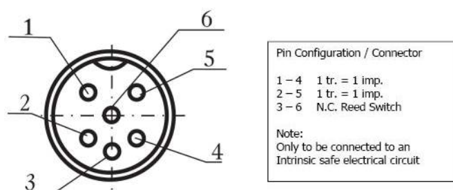
Figure4 Mechanical index with LF output
